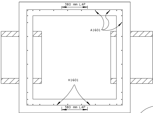
SECTION E-E
